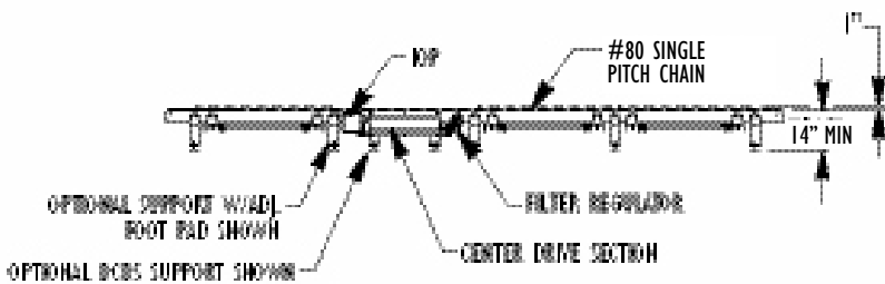
VIEW X-X
