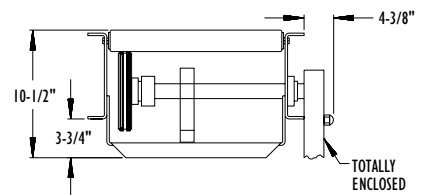
SECTION "Y-Y"
