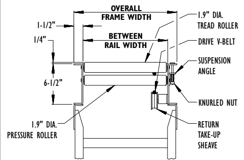
SECTION "X-X"
